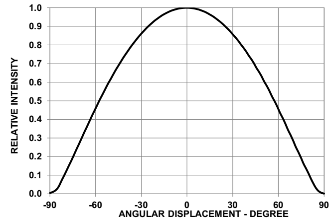
Figure 6 Radiation Pattern
