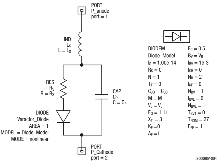
Figure 4. SPICE Model
