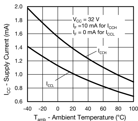
Fig. 13 - Supply Current vs. Ambient Temperature
