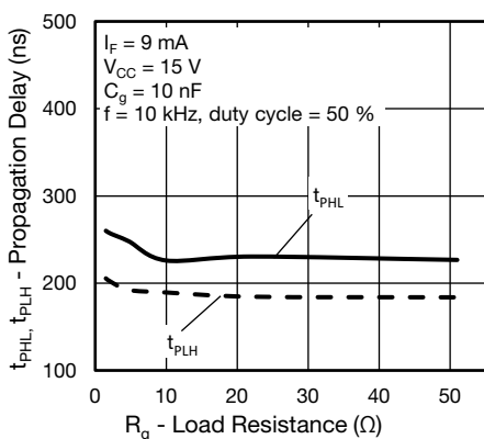
Fig. 20 - Propagation Delay vs. Load Resistance
