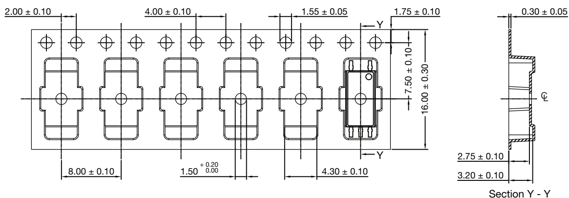
Fig. 26 - Tape and Reel Packing (2000 pieces on reel)
