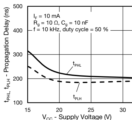
Fig. 17 - Propagation Delay vs. Supply Voltage
