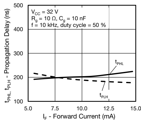
Fig. 19 - Propagation Delay vs. Forward Current
