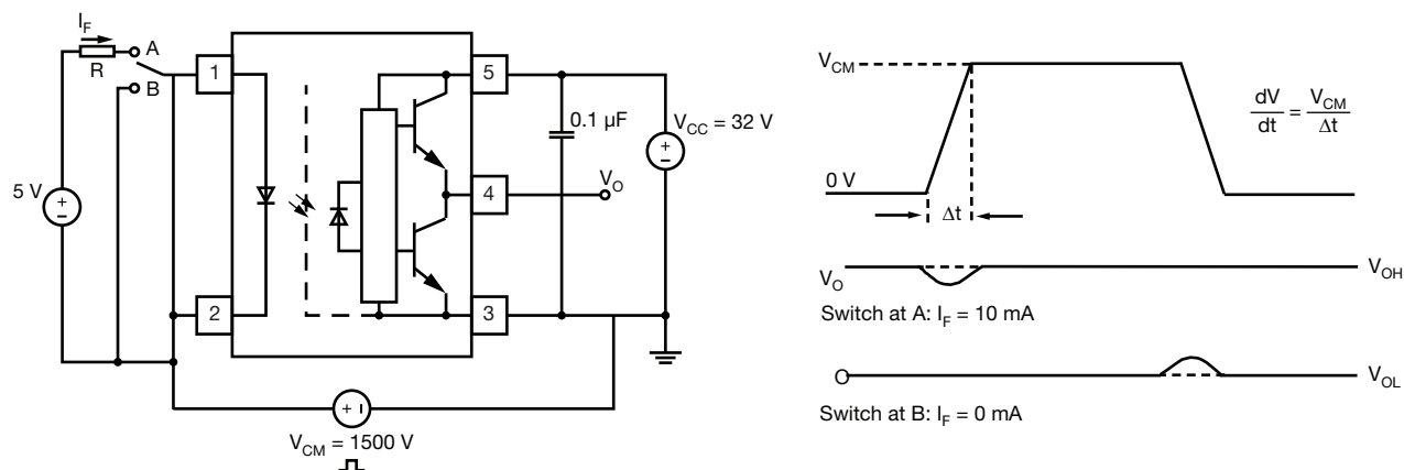
Fig. 5 - CMR Test Circuit and Waveforms
