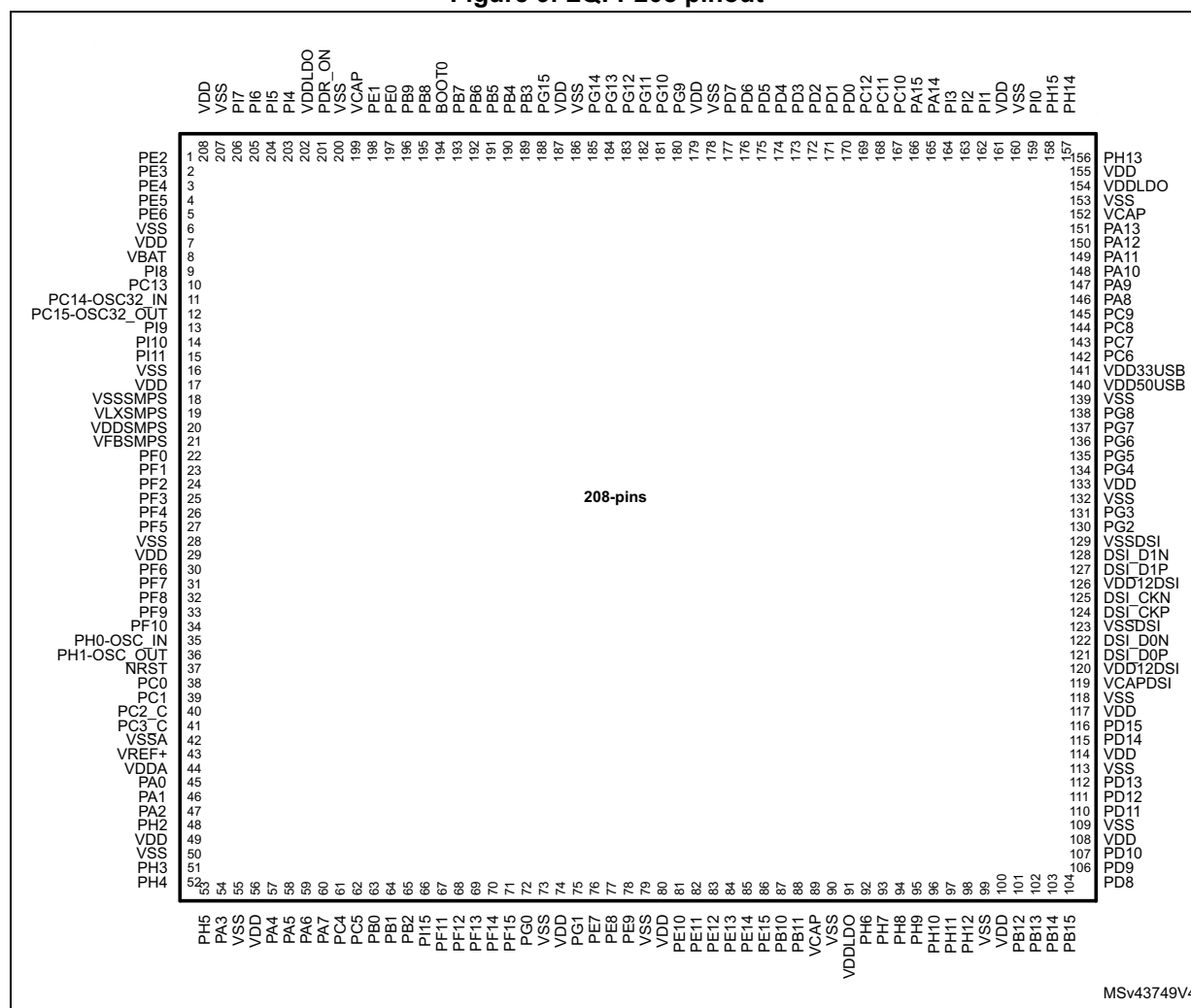
Figure 9. LQFP208 pinout
