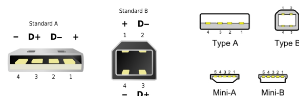
Figure 5 Common USB pin-outs for male connectors
