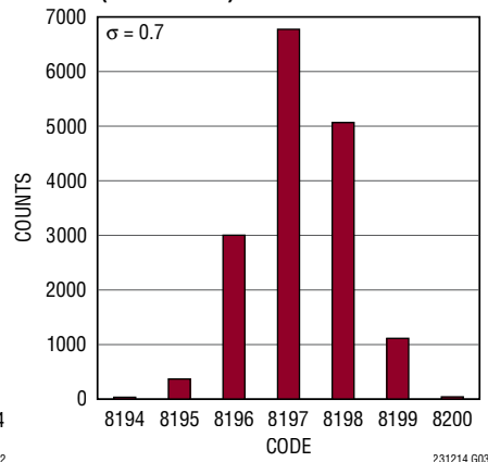
DC Histogram Near Mid-Scale (Code 8192)
