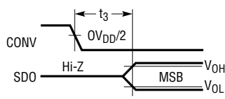
Figure 1. SDO Enabled After CONV↓
