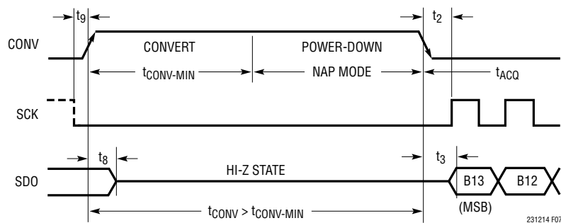
Figure 7. LTC2312-14 Nap Mode Power-Down Following Conversion for t_{\text{CONV}} > t_{\text{CONV-MIN}}
