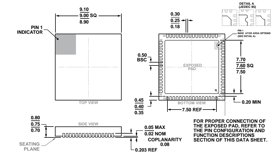
Figure 116. 64-Lead Lead Frame Chip Scale Package [LFCSP] 9 mm × 9 mm Body and 0.75 mm Package Height (CP-64-15) Dimensions shown in millimeters
