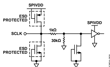
Figure 58. SCLK Input
