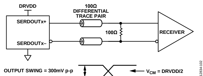
Figure 102. DC-Coupled Digital Output Termination Example
