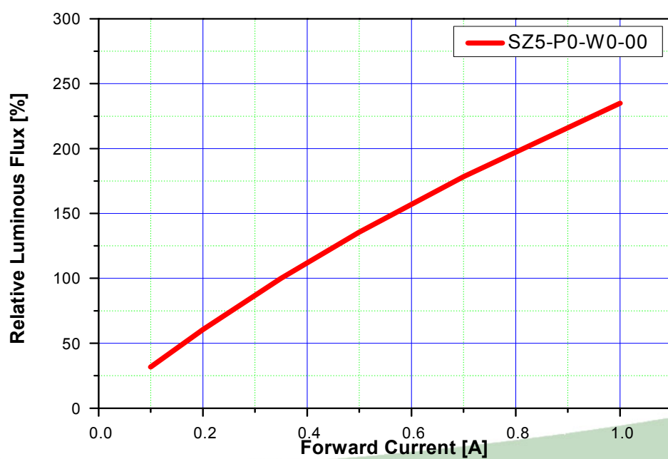
Forward Current vs. Normalized Relative Luminous Flux, T_a = 25^\circ\text{C}
