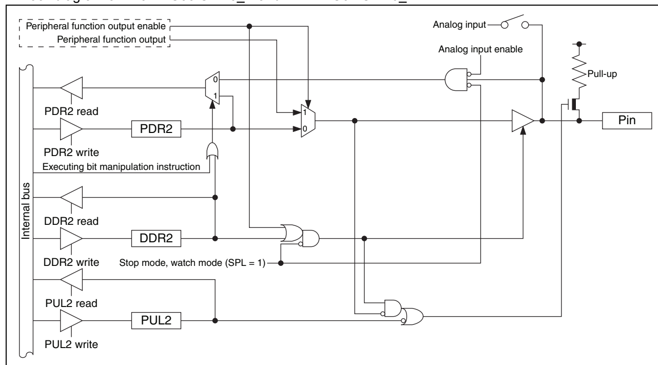
• Block diagram of P20/PPG00/CMP0 N and P21/PPG01/CMP0 P
