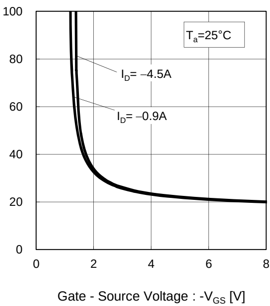
Fig.12 Static Drain - Source On - State Resistance vs. Gate Source Voltage
