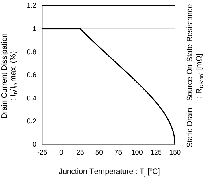
Fig.11 Drain CurrentDerating Curve
