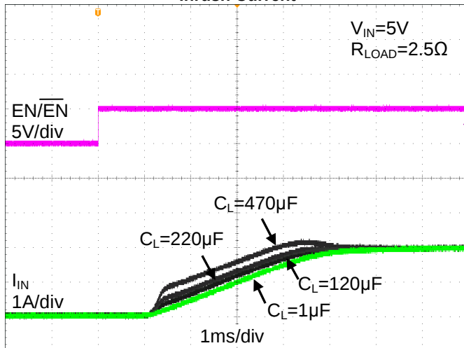
Inrush Current
