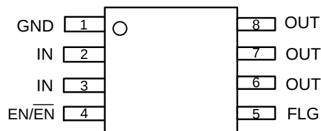
MSOP-8
