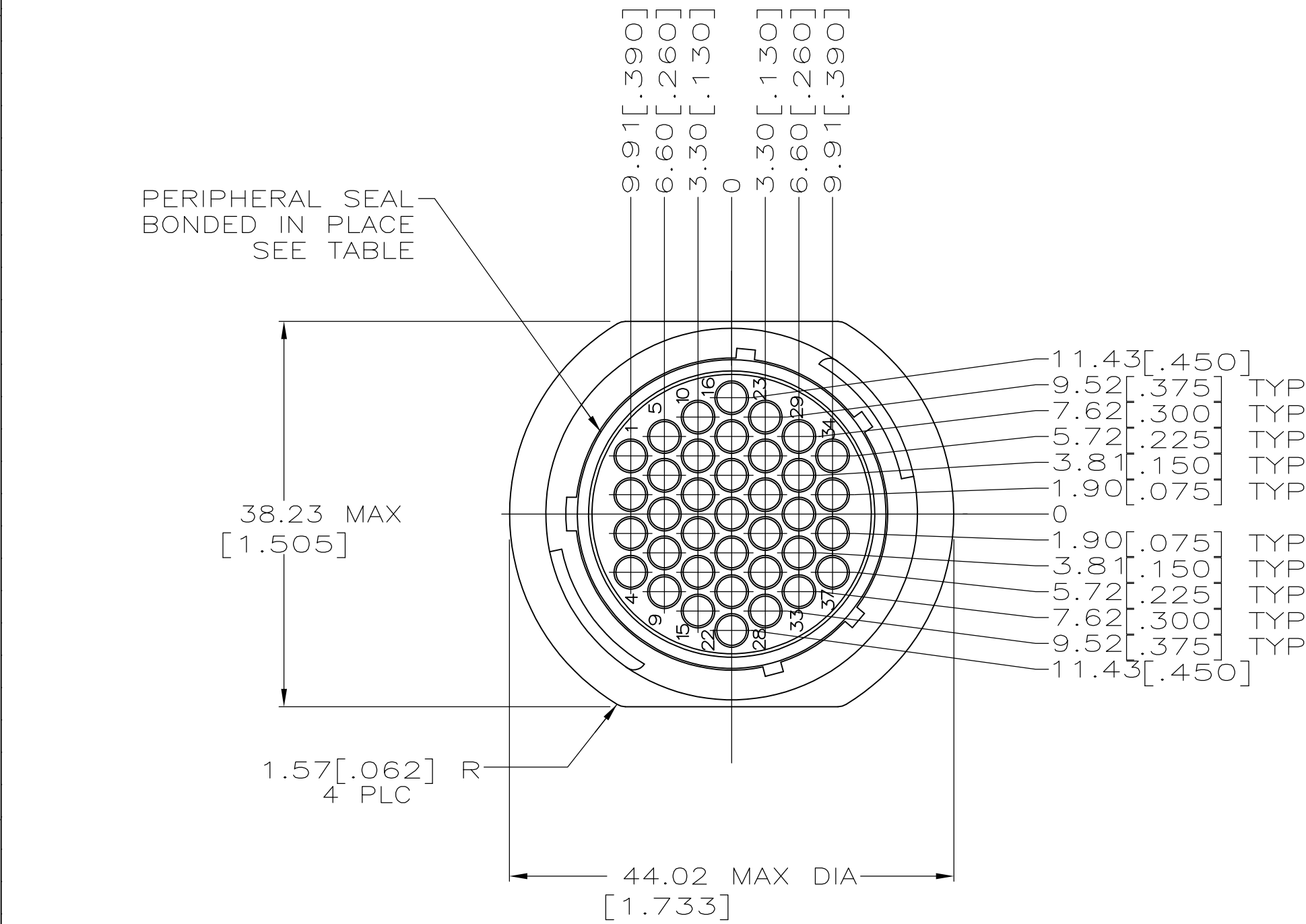
DETAIL B
