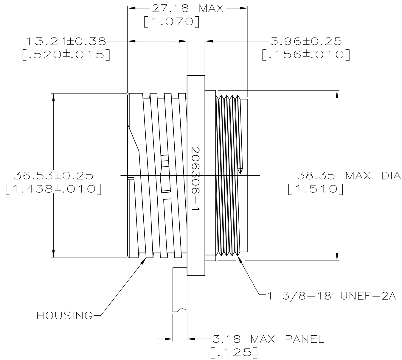
DETAIL A
