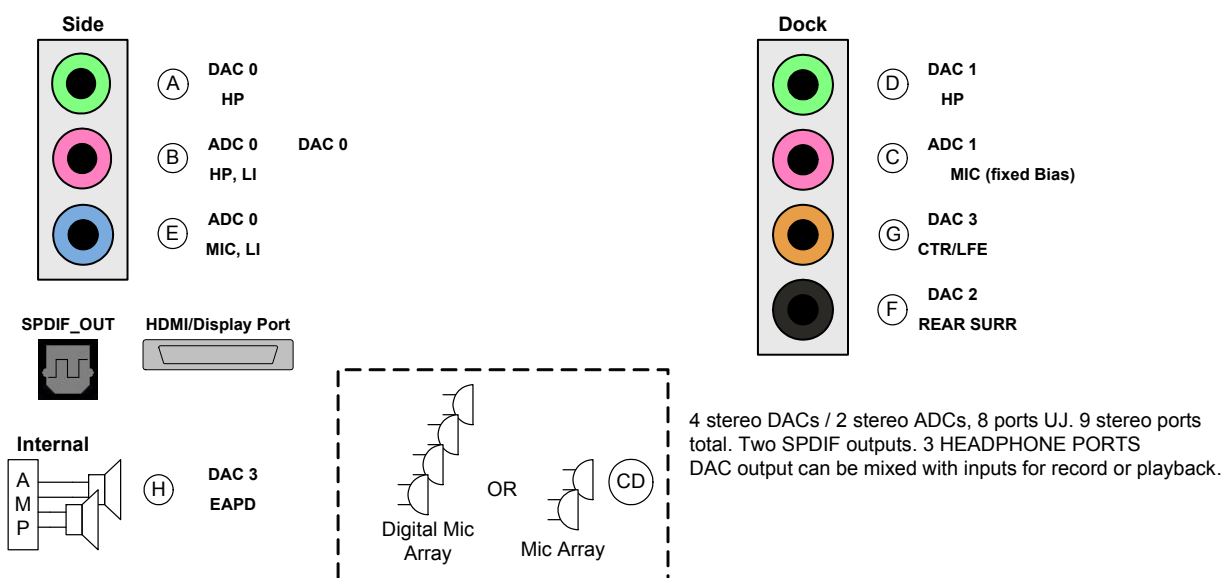
Figure 13. Port Configurations
