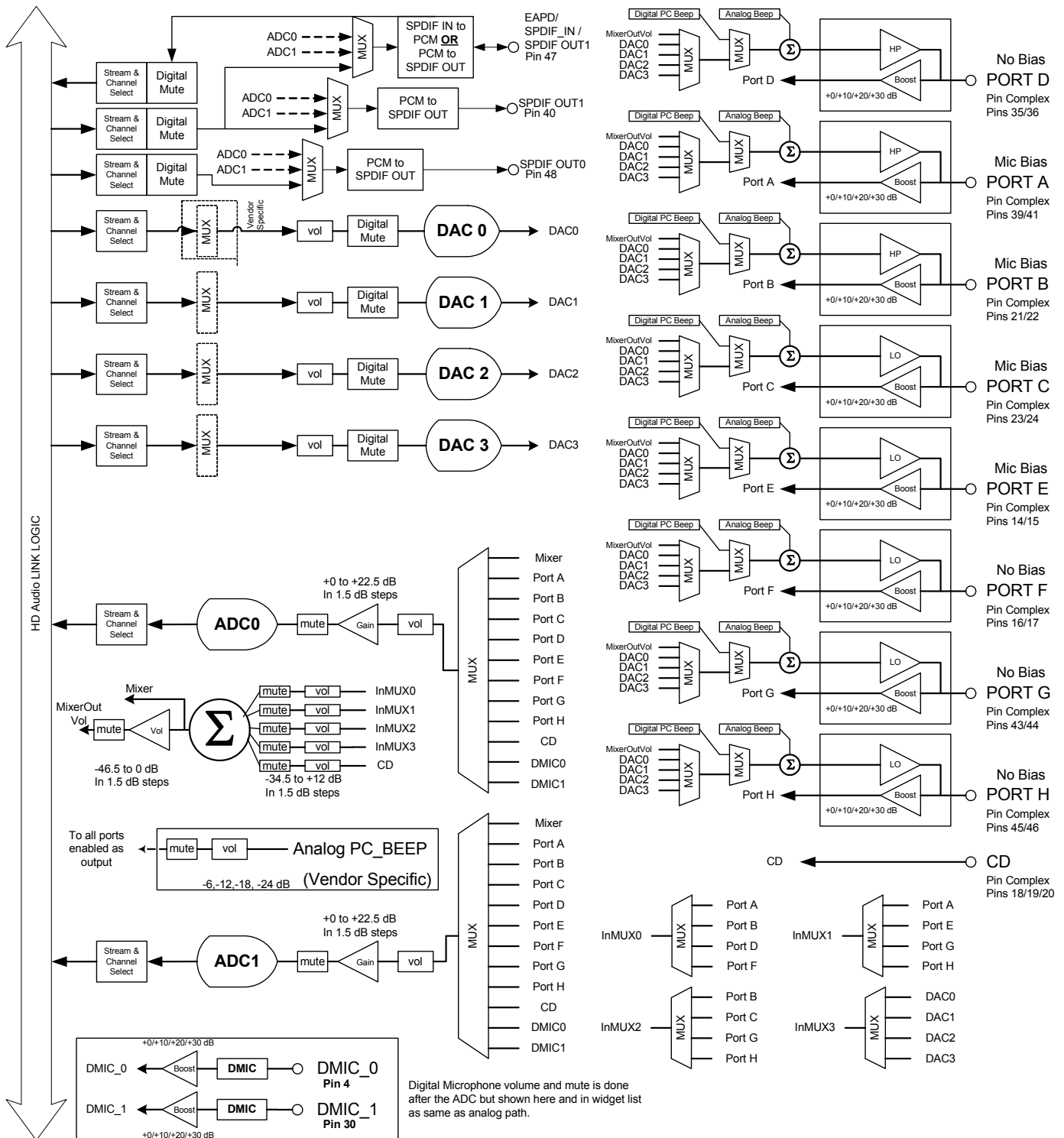
Figure 10. 48QFP Functional Block Diagram
