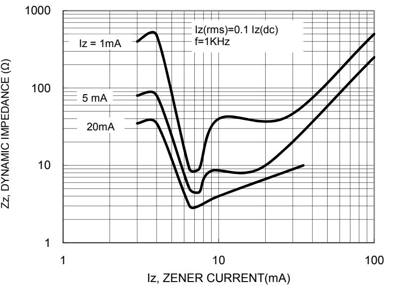
FIG.4 EFFECT OF ZENER VOLTAGE ON ZENER IMPEDANCE
