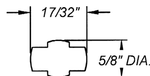
Mounting Hole Diagram
