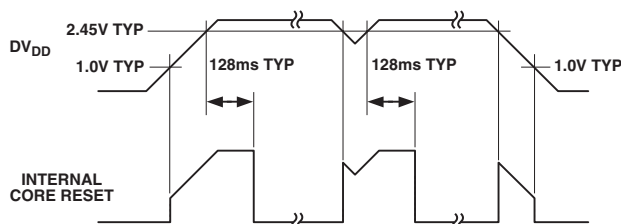
Figure 63. Internal Power-on-Reset Operation
