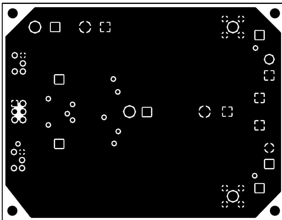
Figure 10. Inner Layer 2
