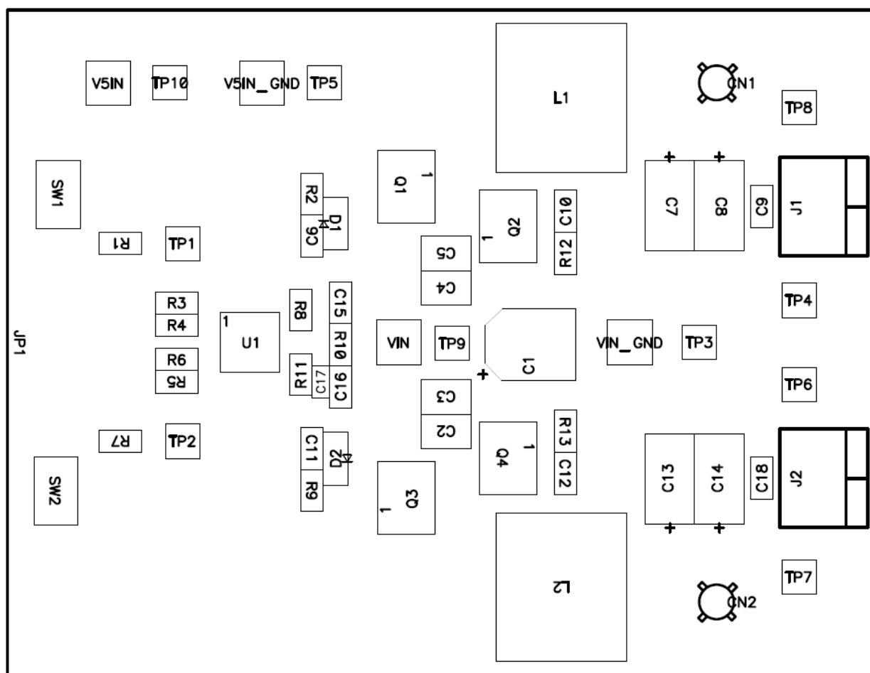
Figure 7. Top Assembly
