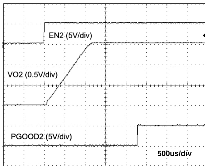
Figure4. 1.5V Startup Waveforms
