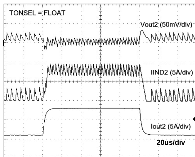
Figure6. 1.5V Load Transient Response
