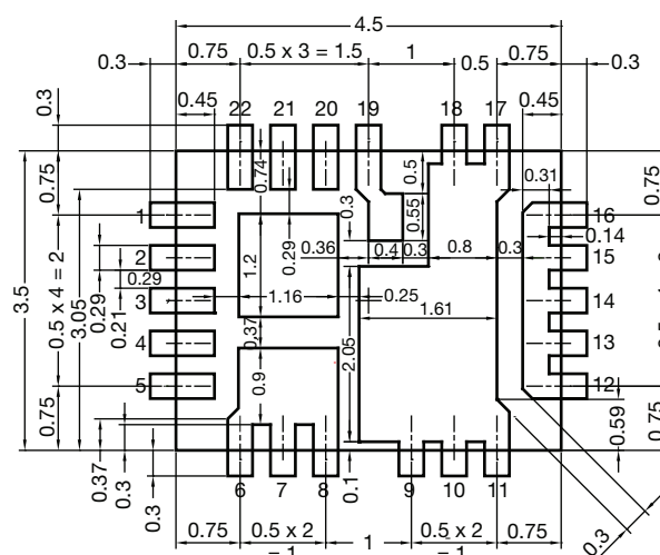
Land pattern
