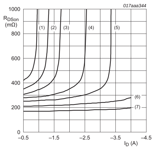
Fig 8. Drain-source on-state resistance as a function of drain current; typical values T_j = 25\text{ °C} (1) V_{GS} = -1.4\text{ V} (2) V_{GS} = -1.5\text{ V} (3) V_{GS} = -1.6\text{ V} (4) V_{GS} = -1.8\text{ V} (5) V_{GS} = -2.0\text{ V} (6) V_{GS} = -2.5\text{ V} (7) V_{GS} = -4.5\text{ V}
