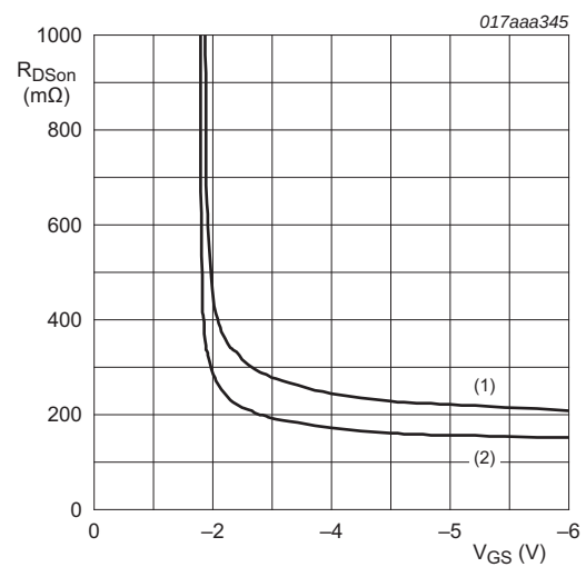
Fig 9. Drain-source on-state resistance as a function of gate-source voltage; typical values I_D = -2.5\text{ A} (1) T_j = 150\text{ °C} (2) T_j = 25\text{ °C}
