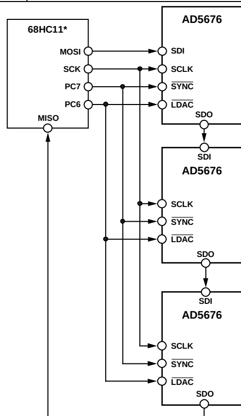
Figure 45. Daisy-Chaining the AD5676
