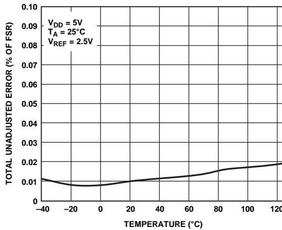
Figure 13. TUE vs. Temperature
