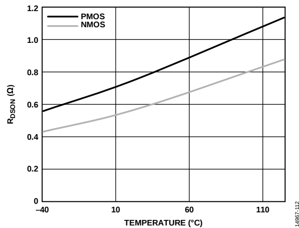
Figure 19. Typical Output Resistance ( R_{DS(on)} ) vs. Temperature, V_{DD2} = 15\text{ V}
