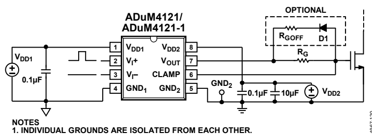
Figure 30. Typical Application Diagram, Single Device
