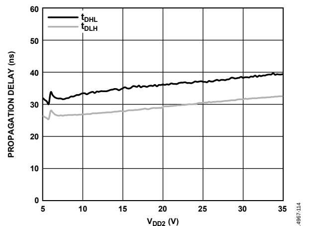
Figure 15. Propagation Delay vs. V_{DD2} , 2 nF Load
