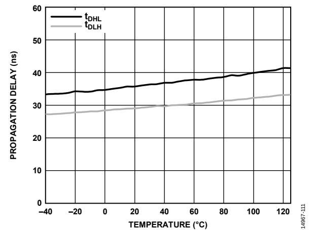
Figure 14. Propagation Delay vs. Temperature, 2 nF Load
