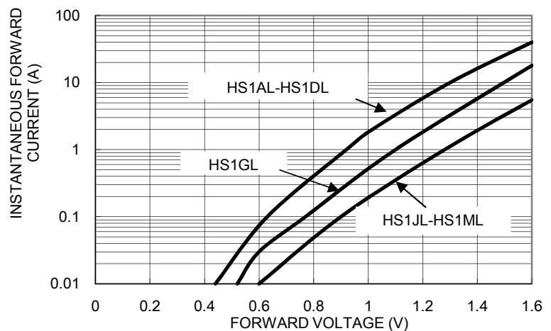
FIG. 4- TYPICAL INSTANTANEOUS FORWARD CHARACTERISTICS
