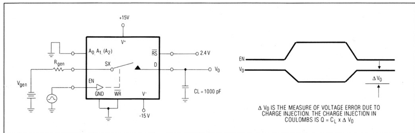
Figure 7. Charge Injection Test Circuit
