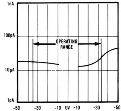
OUTPUT LEAKAGE VS. OFF CHANNEL OVERVOLTAGE WITH \pm 15V SUPPLIES
