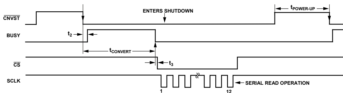
Figure 24. Autos shutdown Mode for AD7366-5
