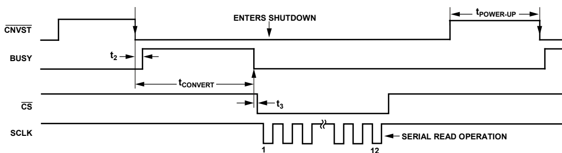
Figure 24. Autos shutdown Mode for AD7366-5
