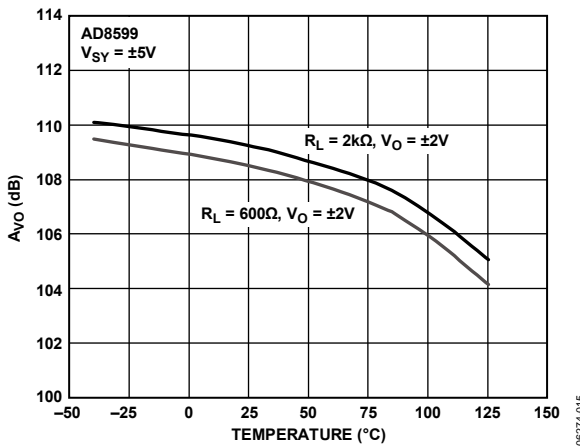
Figure 17. Large Signal Voltage Gain vs. Temperature
