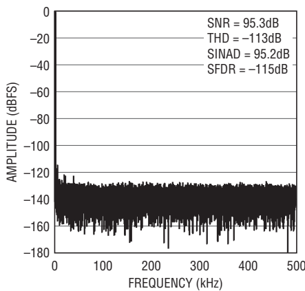
32k Point FFT f_s = 1\text{Mps} , f_{IN} = 2\text{kHz}
