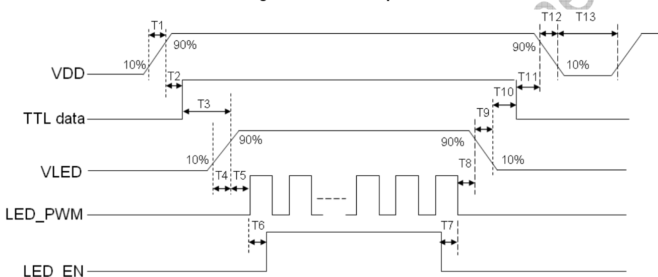
Figure 11 Power Sequence
