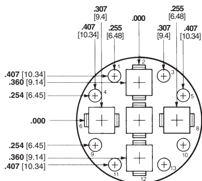
Max. Wire Ins. Dia. = .150 [3.81] for Multimate Contacts, .220 [5.59] for Power Contacts
