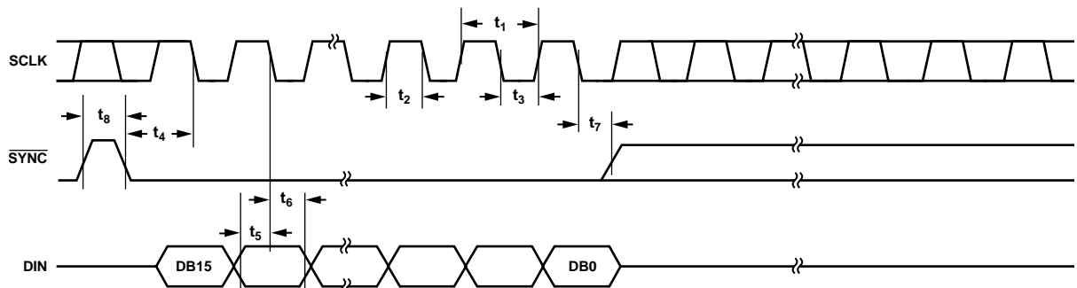
Figure 2. Timing Diagram
