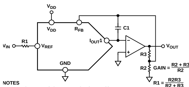
Figure 47. Increasing Gain of Current-Output DAC
