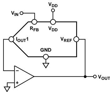
NOTE ADDITIONAL PINS OMITTED FOR CLARITY Figure 48. Current Steering DAC Used as a Divider or Programmable Gain Element
