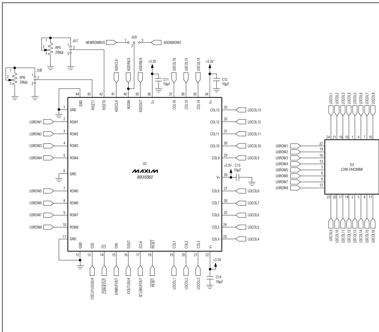
Figure 5. MAX6960 EV Kit Schematic (Sheet 3 of 6)
