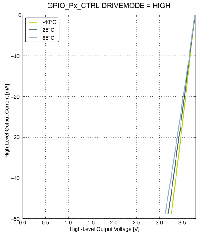
Figure 4.19. Typical High-Level Output Current, 3.8 V Supply Voltage
