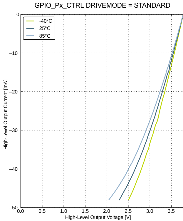
Figure 4.19. Typical High-Level Output Current, 3.8 V Supply Voltage
