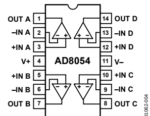
Figure 4. SOIC (R-14) and TSSOP (RU-14)
