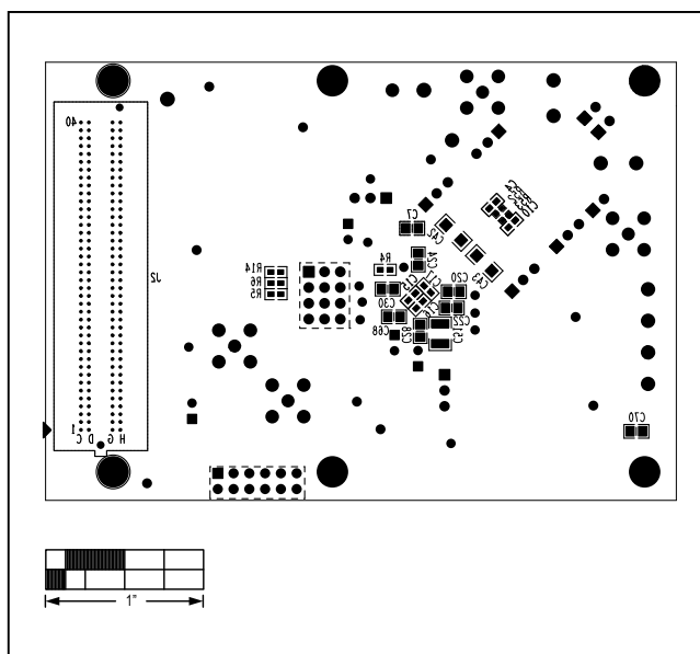
Figure 16. MAX11905 Differential EV Kit Component Placement Guide—Solder Side
