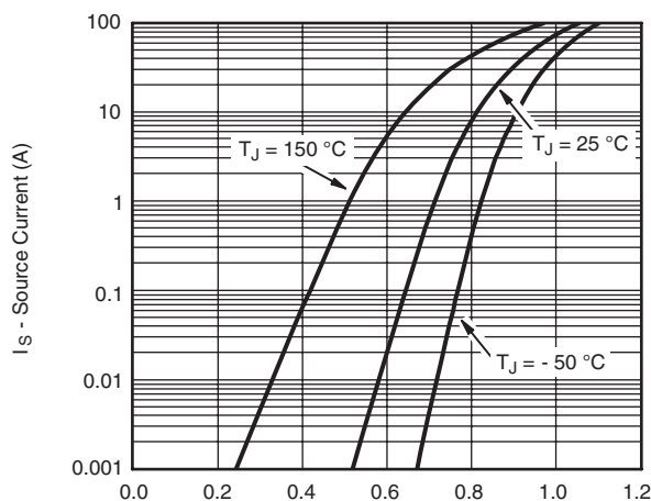
V_{DS} - Source-to-Drain Voltage (V) Source-Drain Diode Forward Voltage
