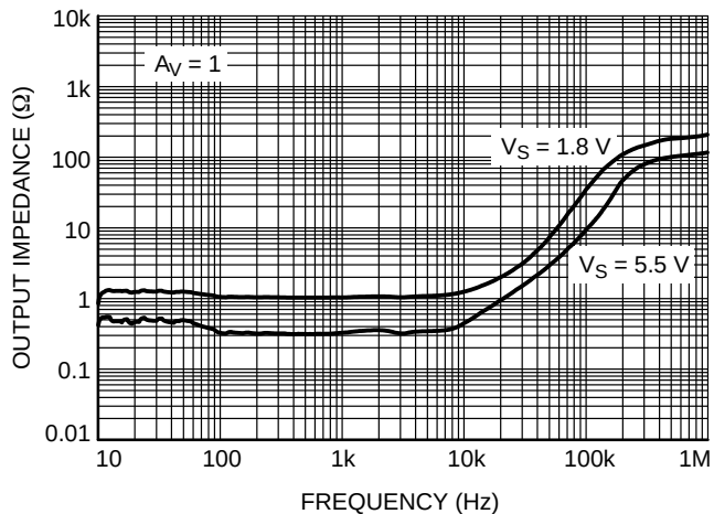
Figure 25. Output Impedance vs. Frequency
