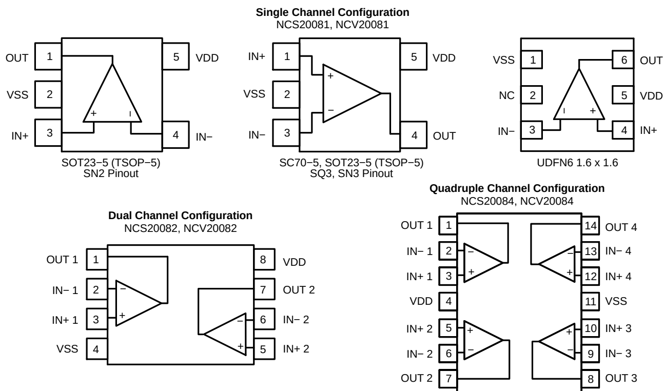
Figure 1. Pin Connections
