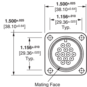
Mating Face
