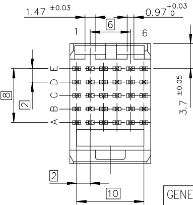
DETAIL-1: PRESS-FIT PIN
