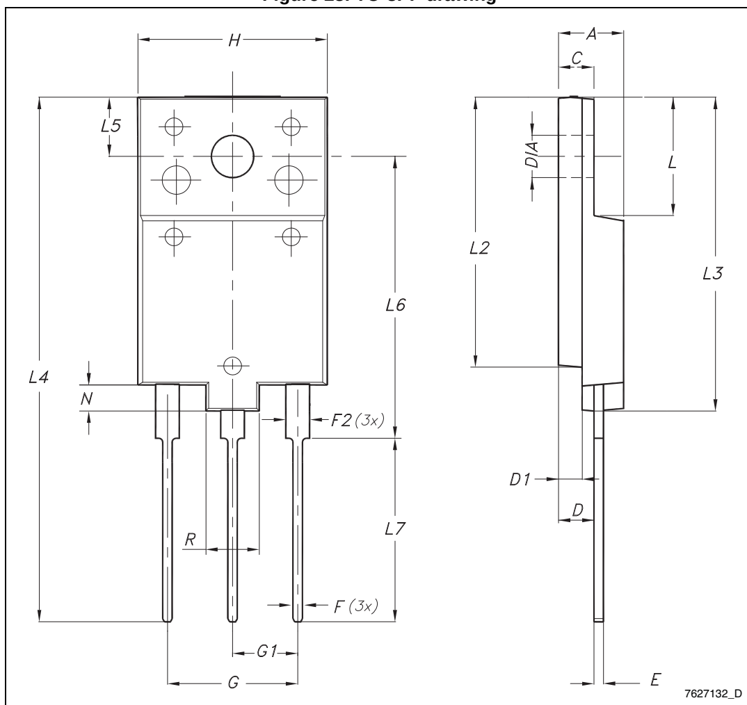
Figure 28. TO-3PF drawing
