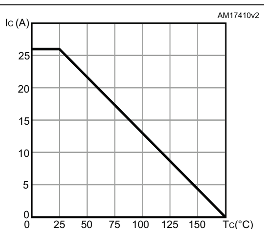
Figure 5. Collector current vs. case temperature for TO-3PF
