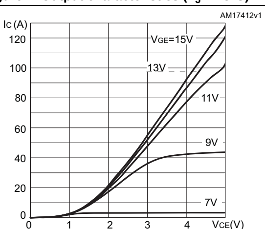
Figure 7. Output characteristics ( T_J=175^\circ\text{C} )
