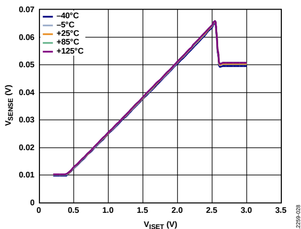
Figure 28. Sense Voltage ( V_{SENSE} ) vs. ISET Voltage ( V_{ISET} ), Different Temperatures
