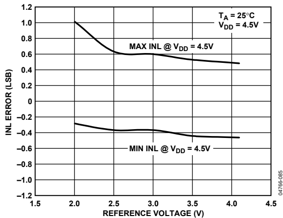
Figure 29. INL vs. V_{REF} @ V_{DD} = 4.5V
